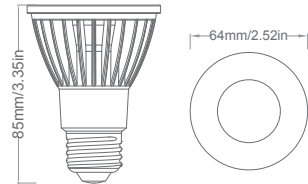
Mechanical Drawing
