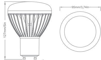
Mechanical Drawing
